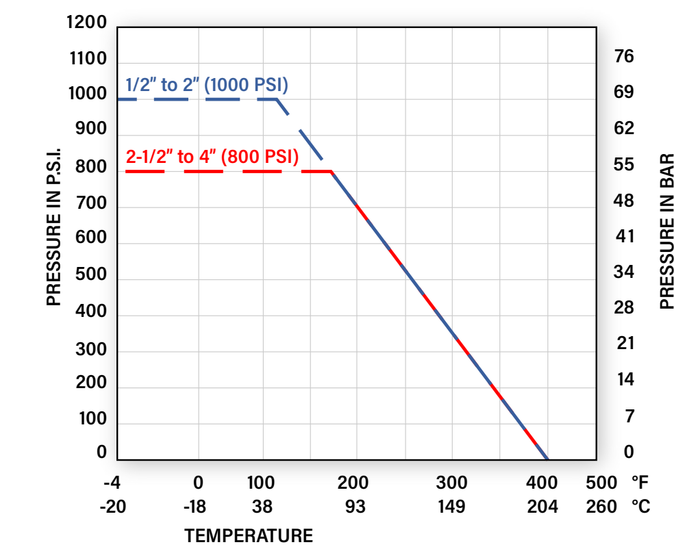
CHART 1: PRESSURE Vs. TEMPERATURE
